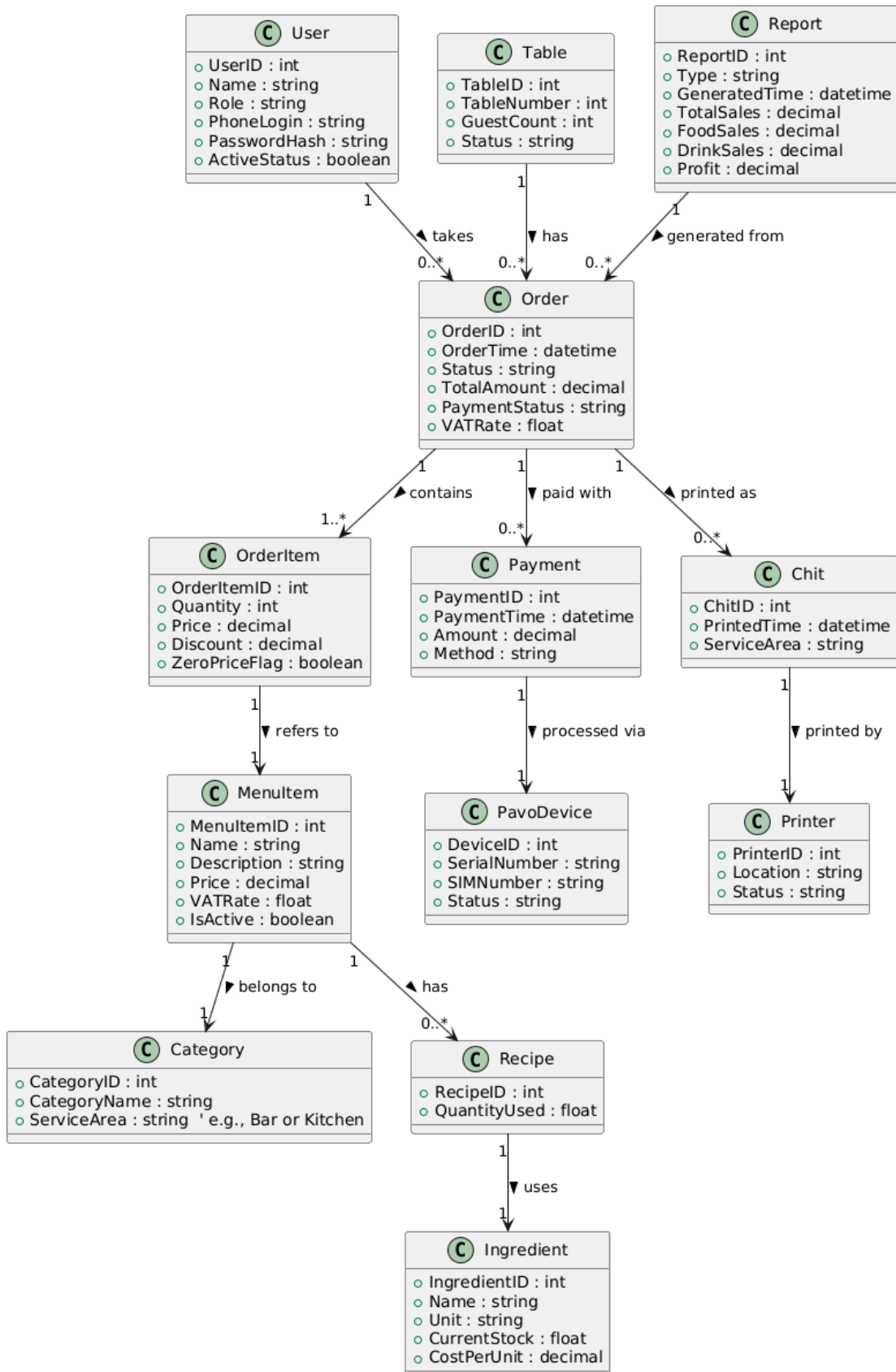
Pionpos System - Irish Luck Pub (ER/UML Diagram)
